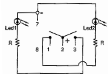
4P SPDT ON-OFF-ON (LED-D)
